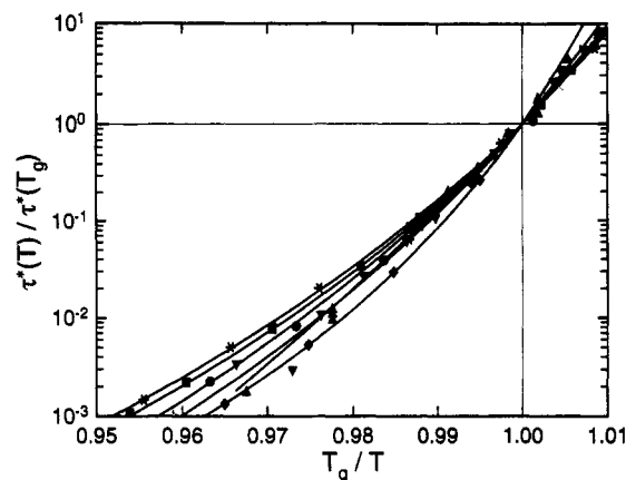
Figure 4. Cooperativity plots corresponding to the Arrhenius curves in Figure 3. The steepest curves are those for PVE networks of highest cross-link density.
