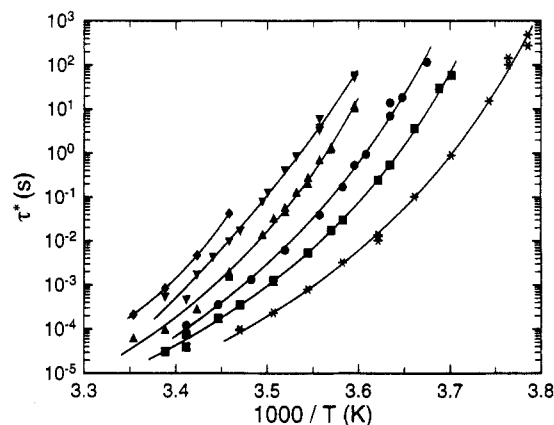
Figure 3. Segmental relaxation times, defined from the peak frequencies, for PVE (symbols as defined in Figure 1), with the fits to eq 5 shown as the solid lines. There is a systematic increase in relaxation time and glass transition temperature with increasing cross-link density.
