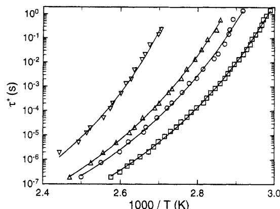
Figure 7. Relaxation times taken as the frequency of the peak for styrene-butyl acrylate copolymers (reported in ref 55). Solid lines represent the Vogel fits (eq 5), and the symbols correspond to 0% (□), 5% (○), 10% (Δ), and 20% (▽) divinylbenzene cross-linker in the polymer backbone.
