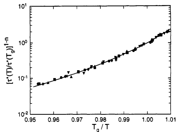
Figure 5. Data in Figure 4 with each curve scaled by the exponent 1 - n (see eq 3). The values for the coupling parameters yielding superpositioning of the data are given in Table 1.
