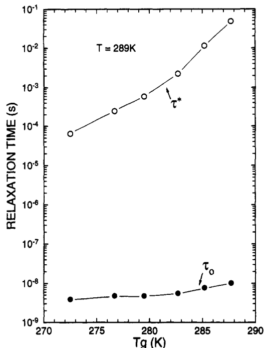
Figure 6. Intermolecularly cooperative ( \tau^* ) and noncooperative ( \tau_0 ) relaxation times for the PVE, with the samples identified by their measured glass transition temperatures (given in Table 1). The \tau_0 's were calculated from the respective \tau^* (measured at T = 289 K) using eq 2 and the value of n determined from construction of Figure 5.
