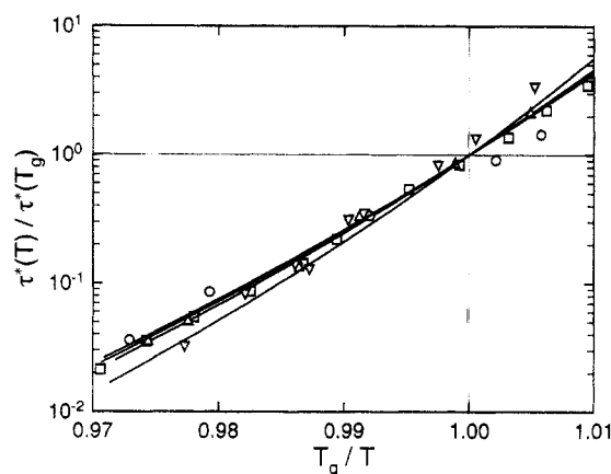
Figure 8. Cooperativity plots constructed from the data in Figure 7, with T_g defined as the temperature at which the peak in the dielectric loss occurs at 10 Hz.
