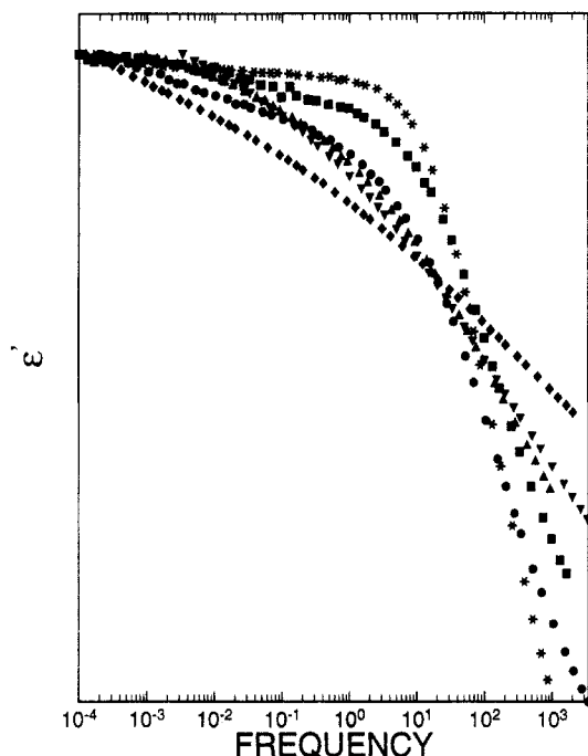
Figure 1. Dielectric constant measured for the linear PVE and the five networks. The data, displayed semilogarithmically, have been vertically scaled and horizontally shifted to facilitate comparison of the shapes in the vicinity of the glass transition. In this and the ensuing Figures 2–5, the symbols correspond to (*) PVE-0, (■) PVE-5, (●) PVE-11, (▲) PVE-22, (▼) PVE-44, and (◆) PVE-66.
