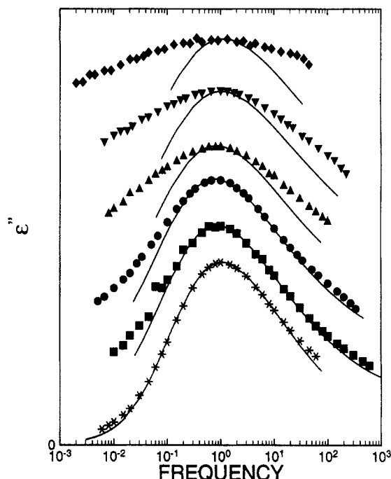
Figure 2. Segmental relaxation dispersion in the dielectric loss for linear PVE and the five networks (symbols correspond to those in Figure 1). The peaks have been arbitrarily shifted to illustrate the systematic broadening accompanying increasing cross-link density. The solid lines were calculated using eq 1, with the values of n determined from superpositioning the cooperativity curves (see Figure 5). The measured experimental dispersions are broader, particularly at the higher cross-link densities, due to inhomogeneous broadening.
